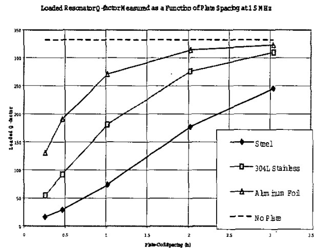
Figure 14. Comparison of Antenna Loading from Steel, Stainless Steel, and Aluminum.
