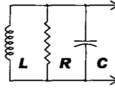
Figure 9. Inductance, L , Capacitance, C , and Resistance, R , of the antenna combine with the metal plate to form a parallel resonant circuit.
