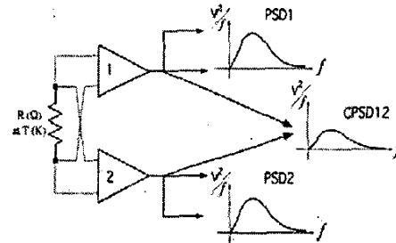
Figure 1. Power Spectral Density Function (PSD) of Each Amplifier Channel Containing Both Correlated and Uncorrelated Noise and the CPSD Function From Both Amplifiers Containing Only Correlated Noise.
