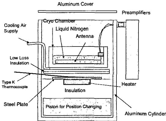
Figure 10. Diagram of Experimental Apparatus Showing Internal Components.
