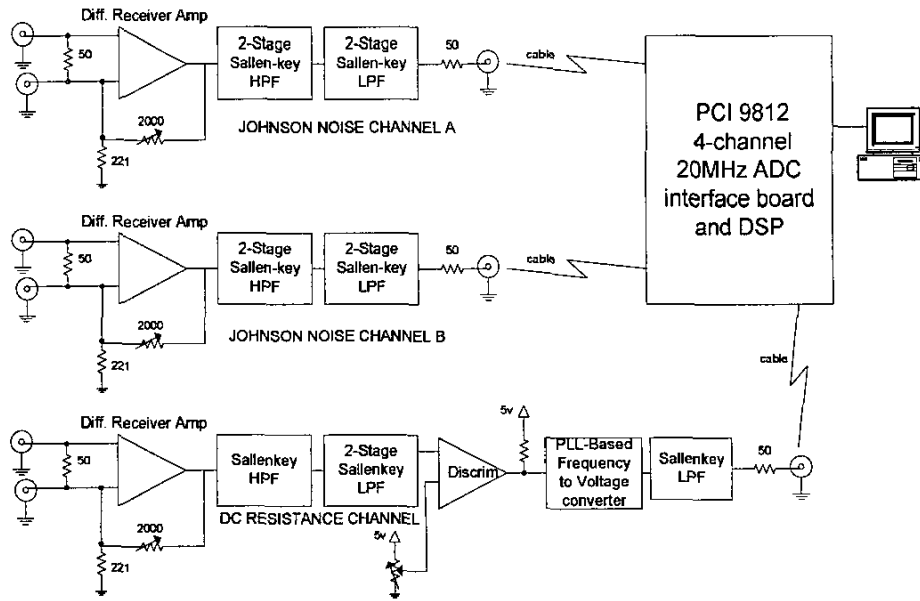
Figure 6. Block Diagram of the Receiver section.
