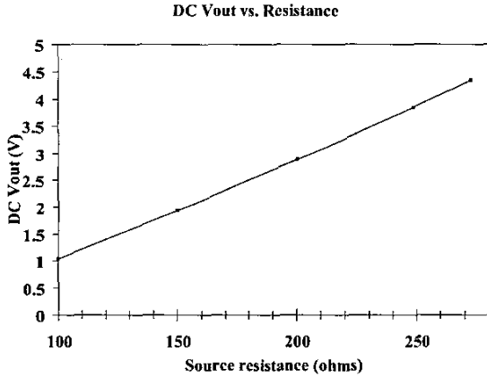
Figure 8. Voltage output versus resistance.
