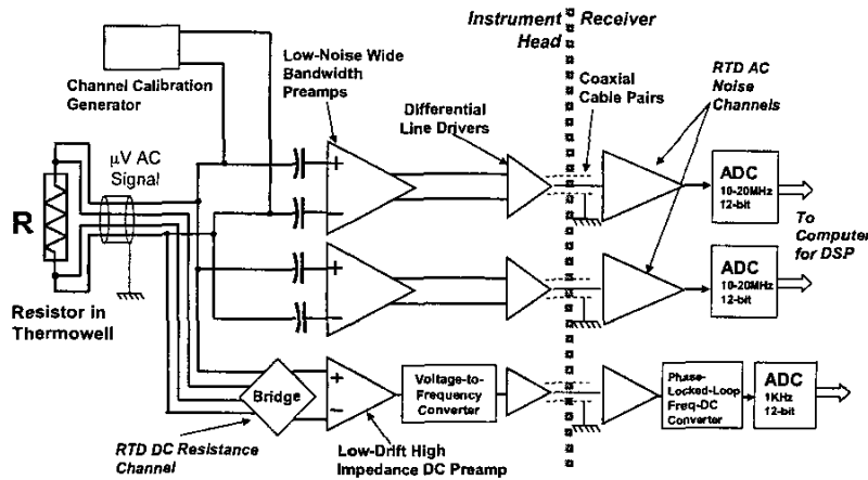
Figure 4. Principal Components And Conceptual Configuration Of The Dual Mode Resistance And Johnson Noise Thermometer Incorporating the Cross-Correlation Technique, Digital Signal Processing, and Channel Gain Calibration.
