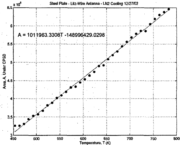
Figure 11. Tracking of Inductive Noise Temperature with Litz Coil Antenna Compared with a Type K Reference Thermocouple.
