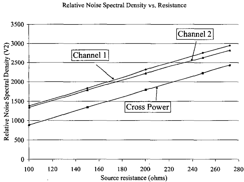
Figure 7. Individual spectral density for each channel and CPSD for both channels versus resistance.
