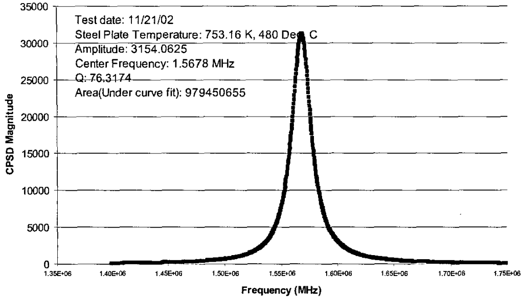
Figure 12. Typical Resonance Curve of the Measured Noise Spectra with Cryogenically Cooled Copper Tubing Coil.
