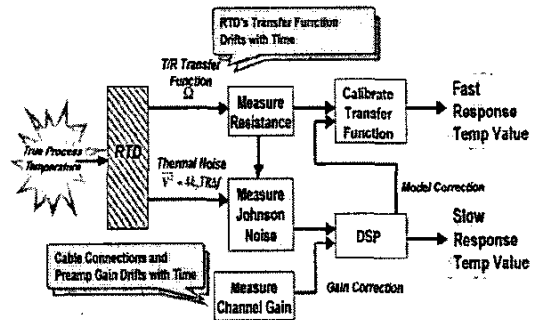
Figure 3. Johnson Noise Thermometry Measurement Process Schematic.
